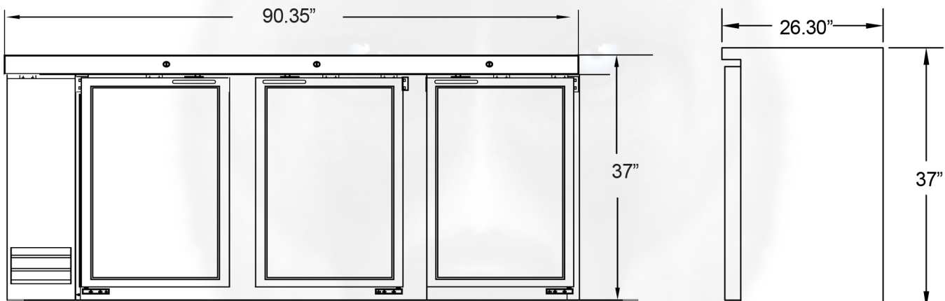
Front View
